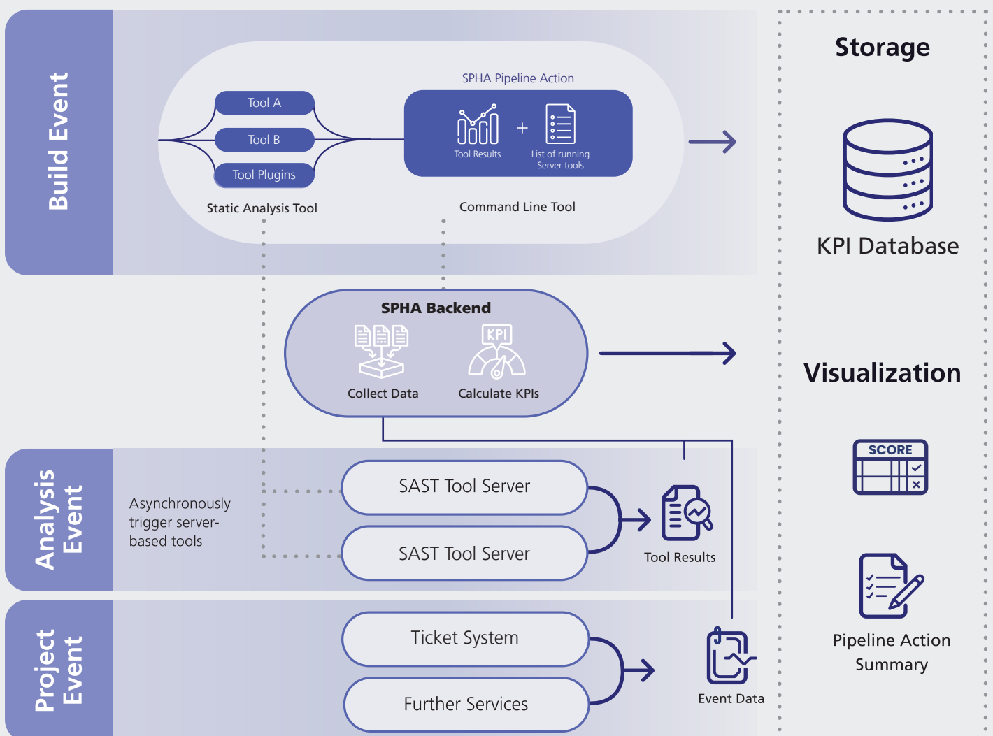
Figure 6: SPHA as a service.
